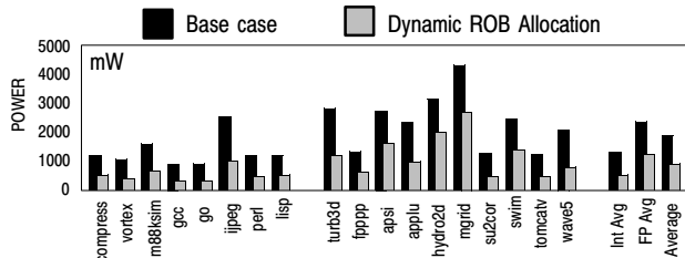
Figure 8. Total power dissipation within the ROB for a 4-way superscalar processor. (Datapath C)
