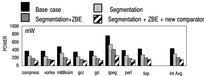
Figure 9. Total power dissipation within DB using bitline segmentation, power efficient comparators and zero-byte encoding (ZBE). (Only SPEC95int results for datapath A are shown)
