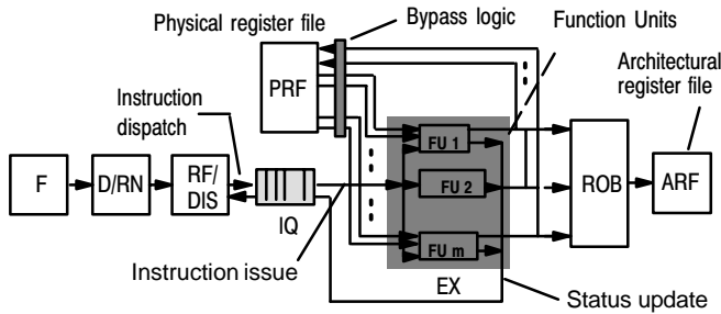
Figure 2. Datapath B
