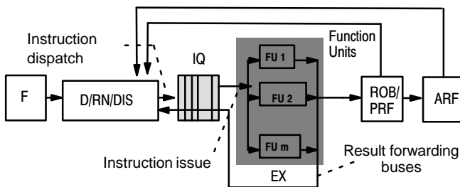
Figure 3. Datapath C
